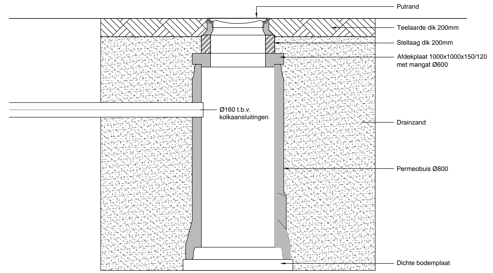
Principedetail Permeoschacht Ø800 Schaal 1:20
